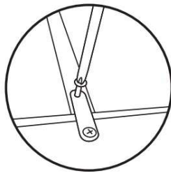
Wall Security Brackets (located installed in wall)
